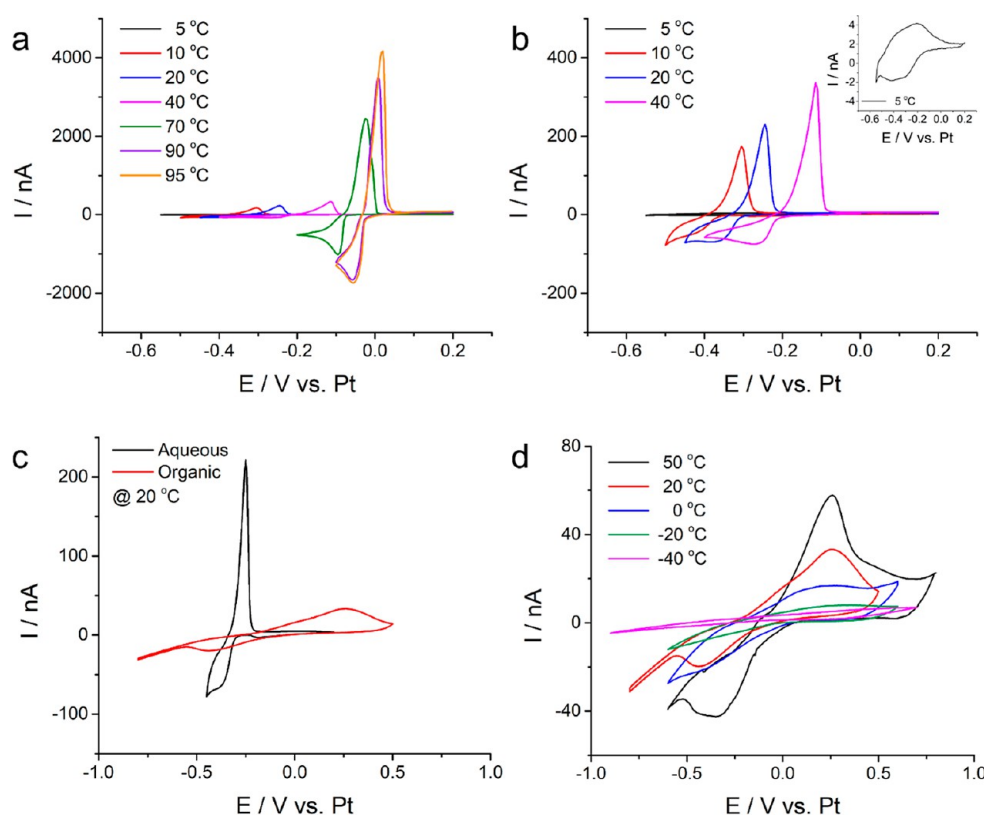
Figure 2. Temperature-dependent Cu electrodeposition/stripping processes in the EC-STEM setup. (a,b) CV profiles in an aqueous solution (10 mM CuSO 4 + 0.1 M H 2 SO 4 ) at 50 mV/s under various controlled temperatures of 5 to 95 °C. The inset shows the CV profile acquired at 5 °C with a redox current of less than 4 nA. (c) CV profiles in an aqueous solution (10 mM CuSO 4 + 0.1 M H 2 SO 4 ) and organic solution (10 mM Cu(OAc) 2 in H 2 O/ethanol (v. 1:1)) at 50 mV/s under the same temperature of 20 °C. (d) CV profiles in the organic solution across a temperature range of -40 to 50 °C at 50 mV/s.
