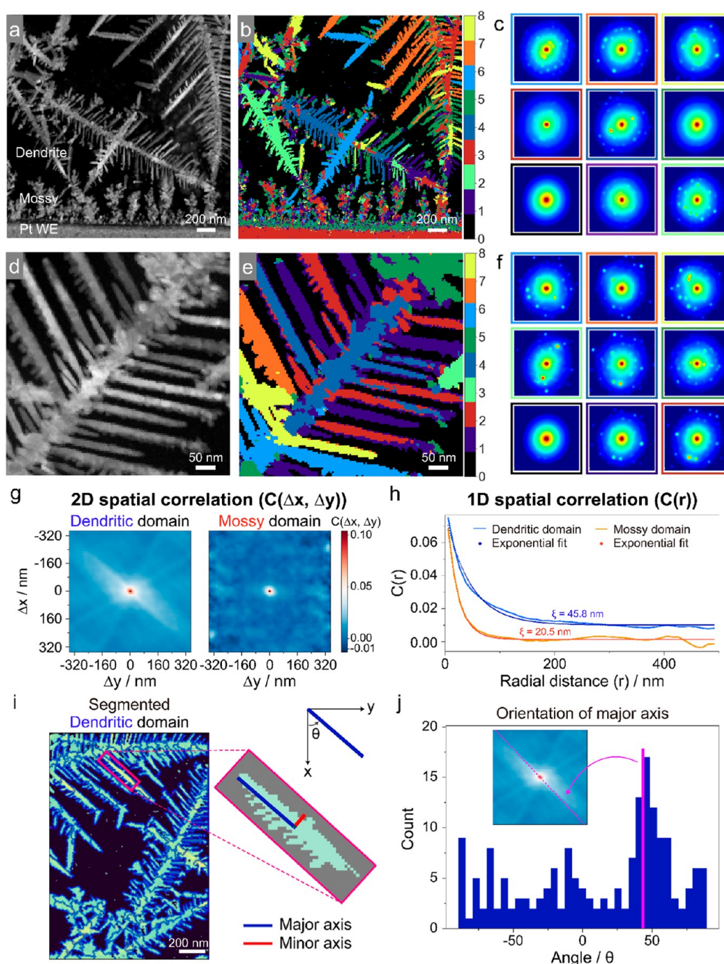
Figure 5. Operando 4D-STEM of Cu dendrites at -40 °C in the organic solution. (a,d) Virtual ADF-STEM image of Cu dendrites grown on the top of mossy Cu and a representative Cu dendrite. (b,c,e,f) False-color 4D-STEM clustering maps of dendritic and mossy Cu structures and corresponding electron diffraction patterns in various colors showing different crystal orientations. (g) 2D spatial correlation functions of Cu nanograins in dendritic (left) and mossy domains (right). (h) 1D spatial correlation functions and their exponential fits in dendritic and mossy domains. (i) Segmentation of dendrites and their ellipse fits for extracting orientation of their major axis. (j) A histogram for orientations of the major axis from the ellipse fit of segmented dendrites.
